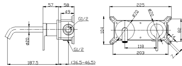
REF. 68437 Ø 35
