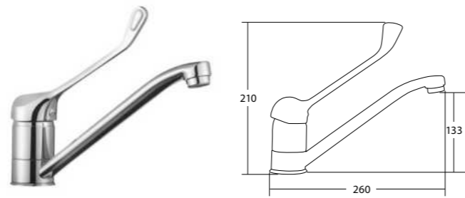
REF. 14053 Ø40
