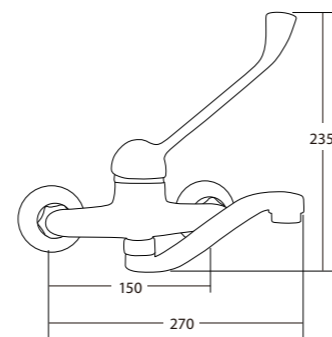
REF. 14054 Ø 40
