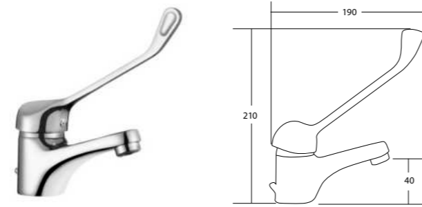
REF. 14052 Ø 40
