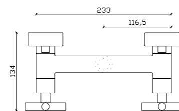
REF. 68024 Ø 1/2
