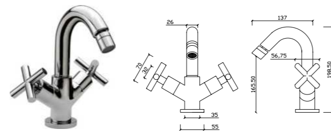
REF. 68022 Ø 1/2
