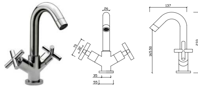
REF. 68021 Ø 1/2
